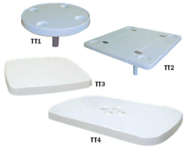
TT1 Circular table top. 58cm diameter TT2 Fold up table top. 76 x 74 cm TT3 Square table top. 78 x 78 cm TT4 Rectangular table top with insert for drinking glasses etc. 123 x 74 cm
